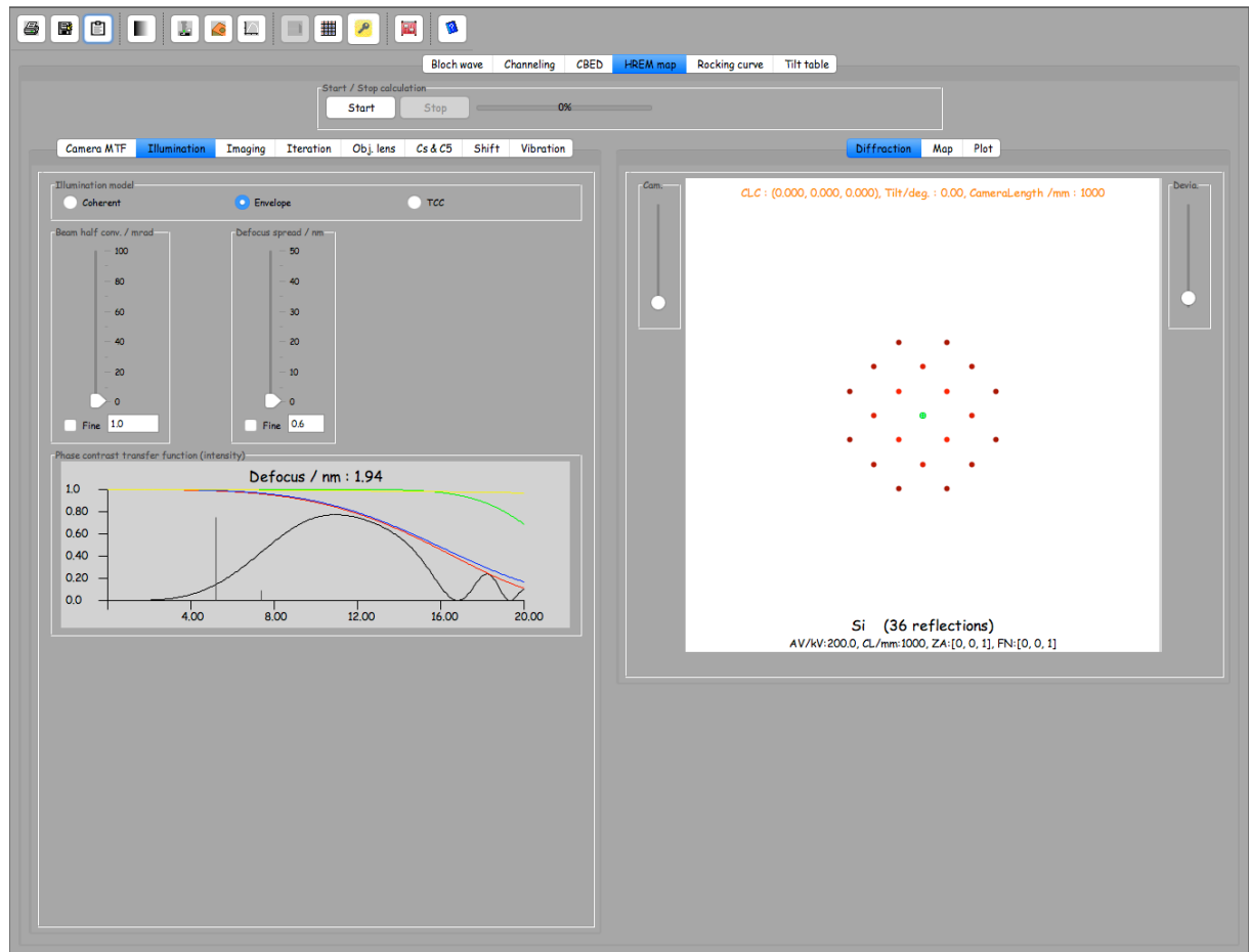
Figure 4: HREM tab
