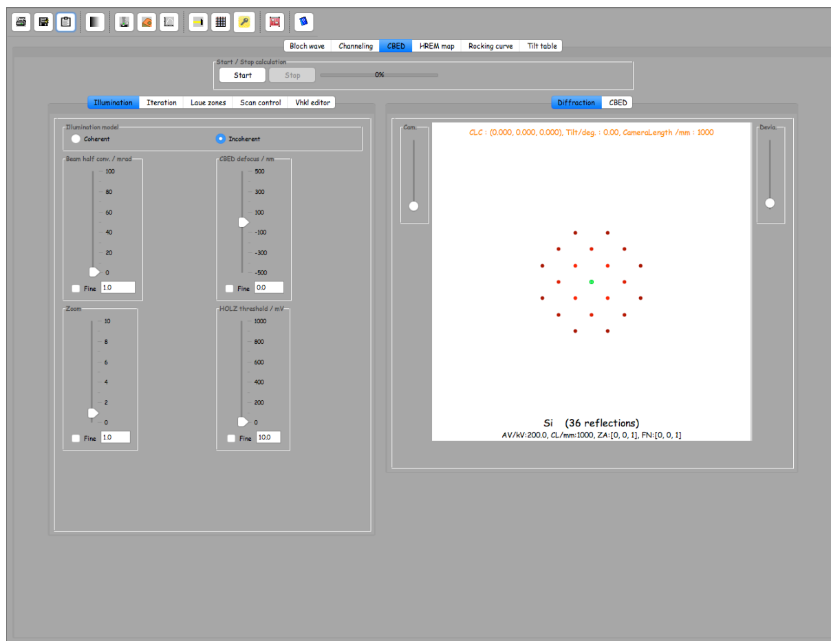
Figure 3: CBED tab
