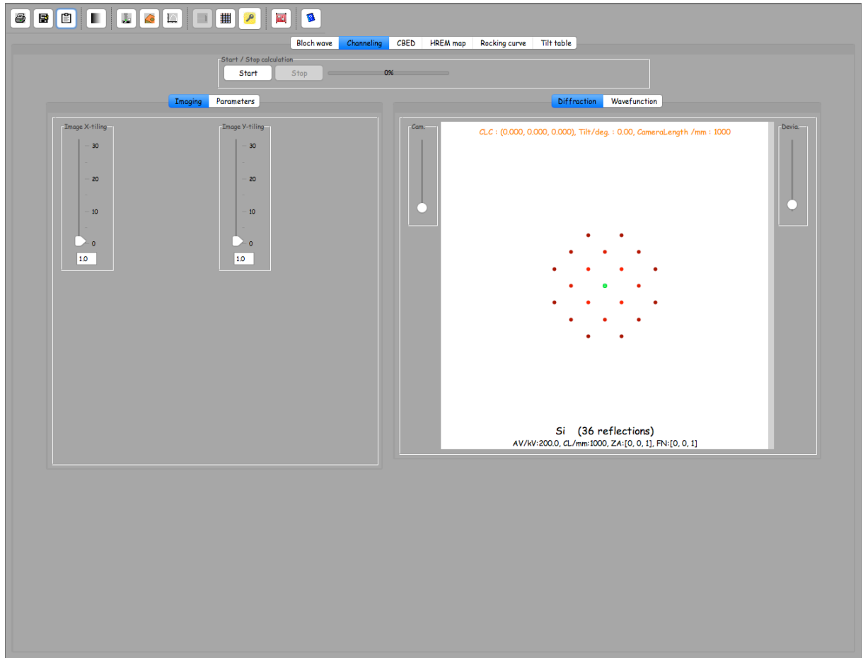
Figure 2: Chenneling tab
