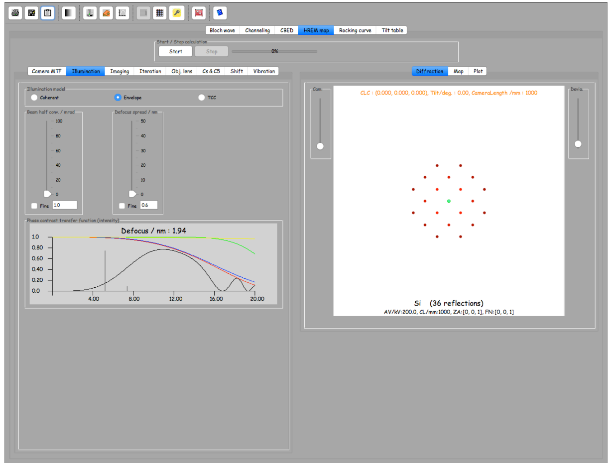
Figure 5: RockingCurve tab
